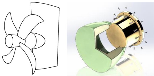
Figure 2: Structure of Ultimate Rudder Bulb
