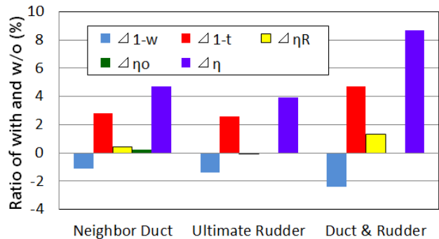
Figure 7: Model test results of combined condition
