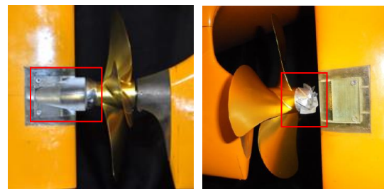
Figure 4: Ultimate Rudder Bulb and ECO-Cap
