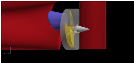
Figure 9: Propeller and energy saving devices for CFD
