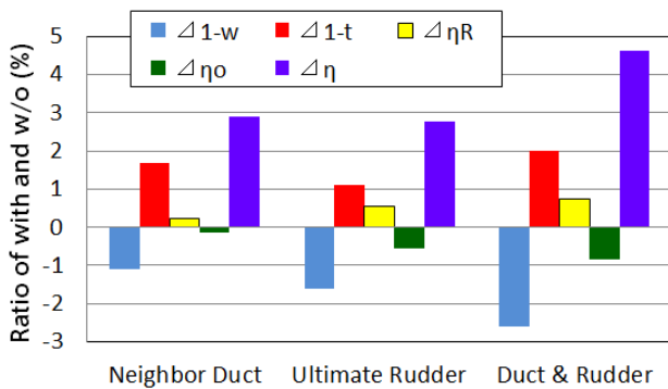
Figure 10: Analysis results of combined condition
