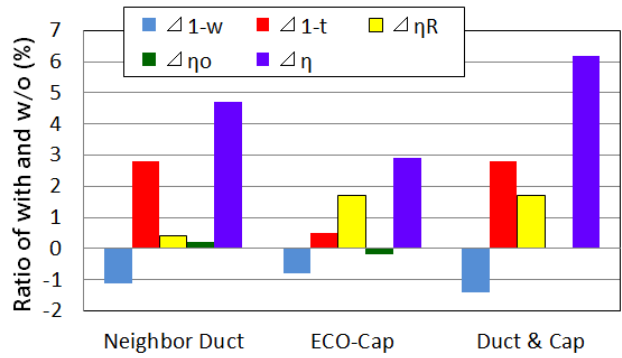
Figure 6: Model test results of combined condition
