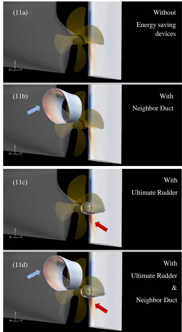
Figure 11: Comparison of pressure distribution
